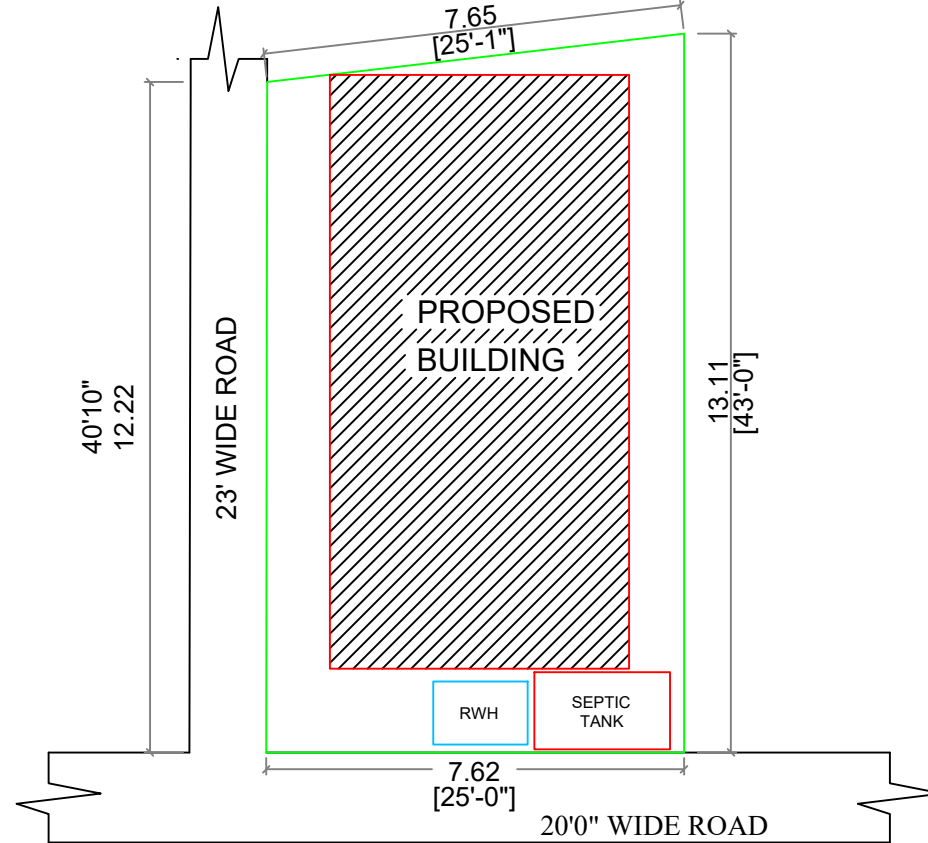
SITE PLAN
