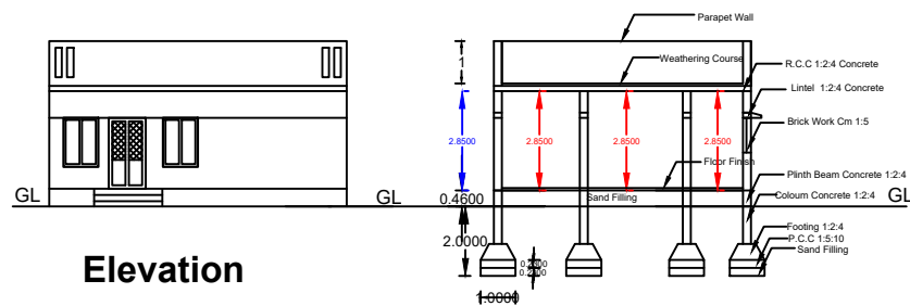
Section Section - AA
