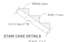
STAIR CASE DETAILS
