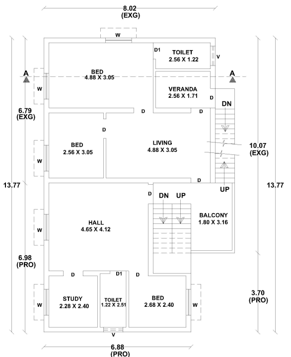
EXG. & PRO. FIRST FLOOR PLAN
