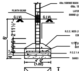
FOUNDATION DETAIL
