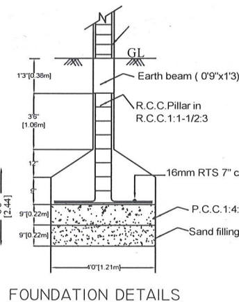
FOUNDATION DETAILS
