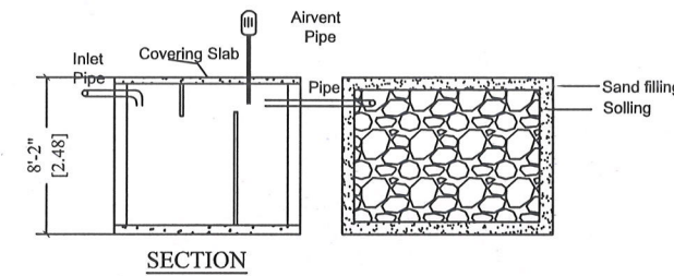
DETAILS OF SEPTIC TANK & DISPERSION TRENCH
