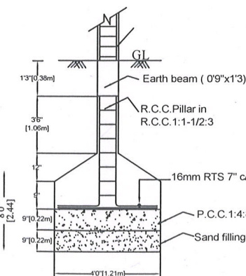
FOUNDATION DETAILS
