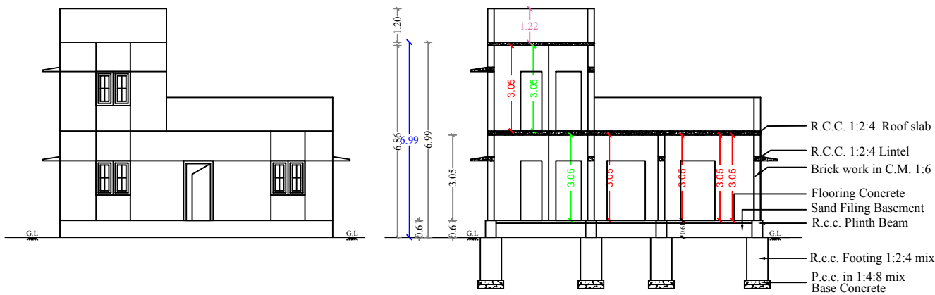
FRONT ELEVATION
