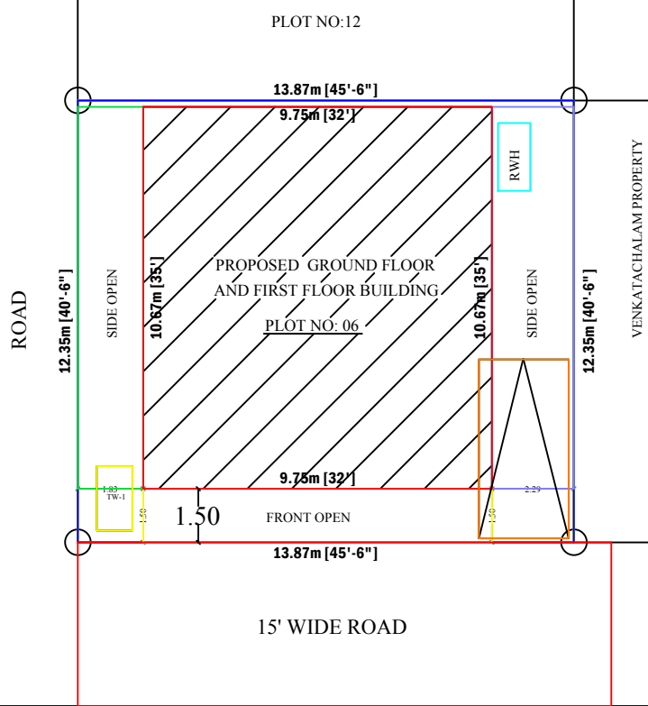
SITE PLAN
