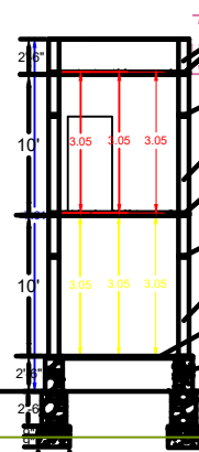
SECTION ON AA'
