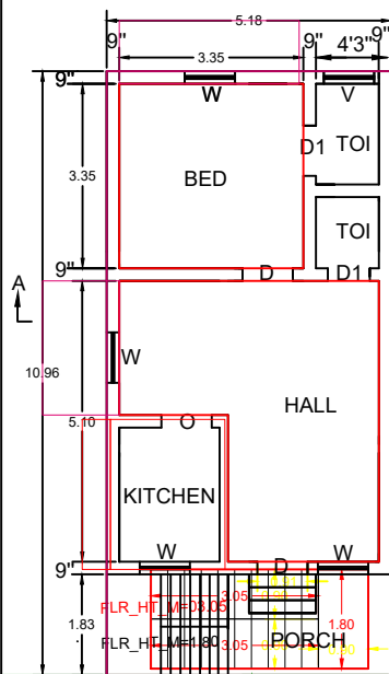
PROPOSED G.F PLAN
