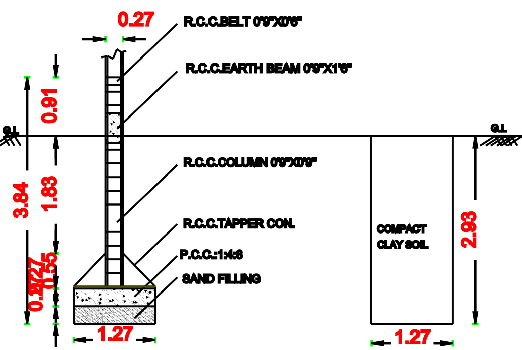
FOUNDATION DETAILS-MIDDLE COLUMN
