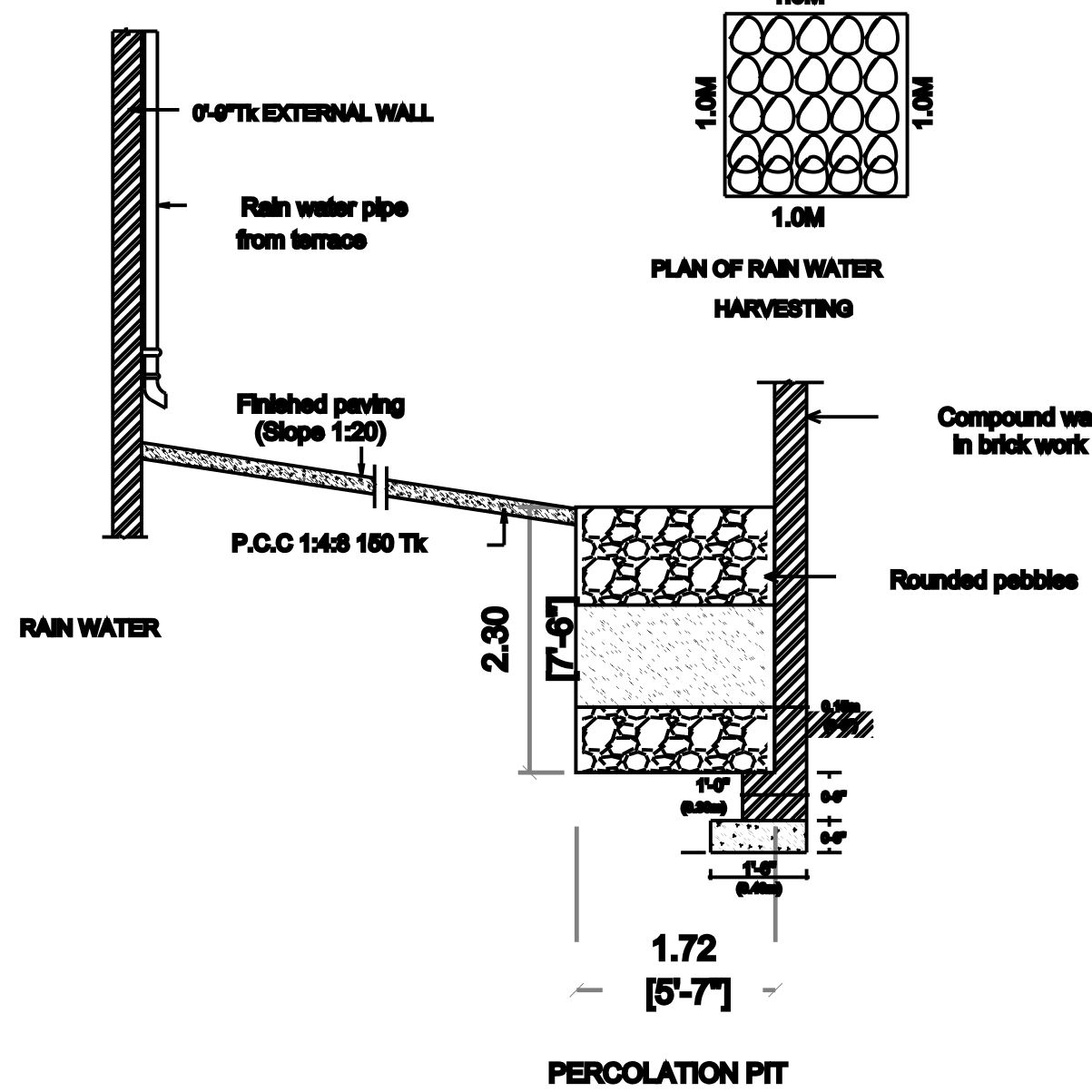
PERCOLATION PIT
