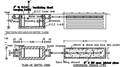
DETAILS OF SEPTIC TANK & DISPERSION TRENCH
