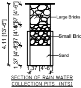
SECTION OF RAIN WATER COLLECTION PITS (NTS)
