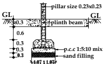
FOUNDATION DETAILS
