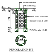
PERCOLATION PIT
