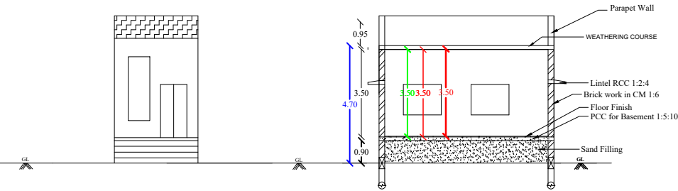
SECTION ON-AA
