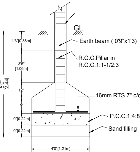
FOUNDATION DETAILS
