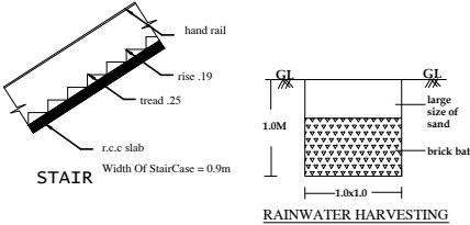
RAINWATER HARVESTING
