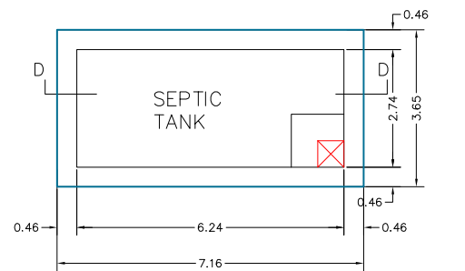
PLAN OF SEPTIC TANK SCALE 1"=2'0"
