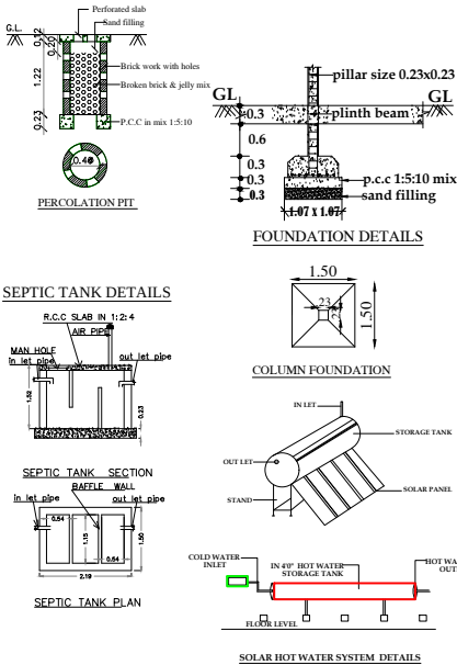
SOLAR HOT WATER SYSTEM DETAILS
