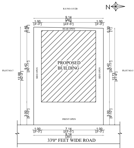
SIDE PLAN
