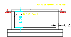
RWHS_SECTION (SAMPLE) RWHS_CAPACITY_L = 2000LTRS
