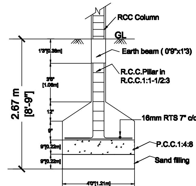
FOUNDATION DETAILS
