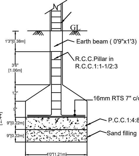
FOUNDATION DETAILS
