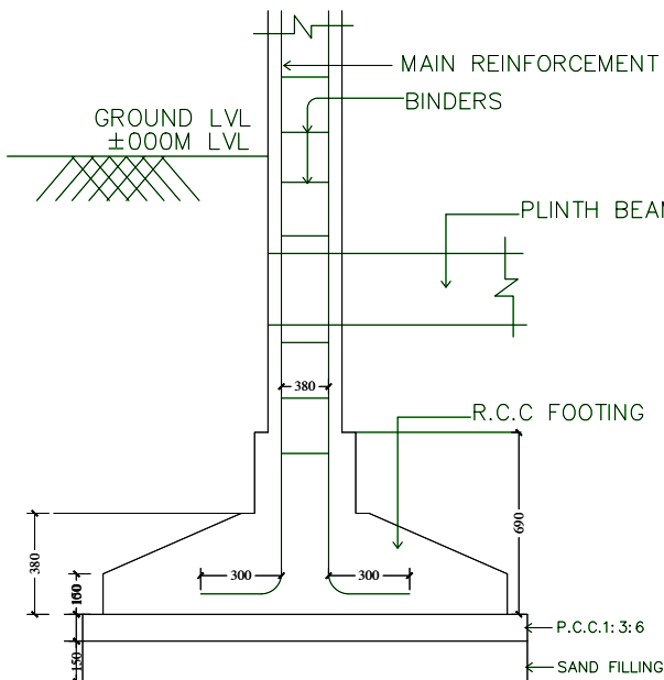
TYPICAL SECTION OF R.C.C. COLUMN FOUNDATION SCALE : 1" = 2'-0"
