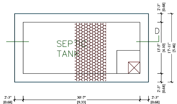
PLAN OF SEPTIC TANK SCALE 1"=2'-0"
