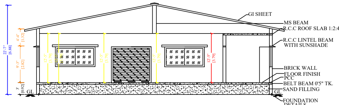
SECTION ON AA- WEST FACING
