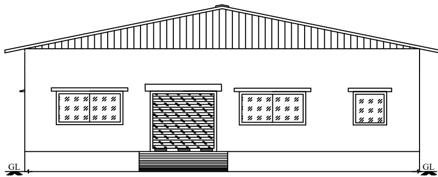
ELEVATION - WEST FACING
