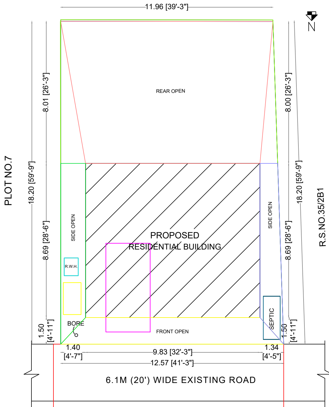
SITE PLAN
