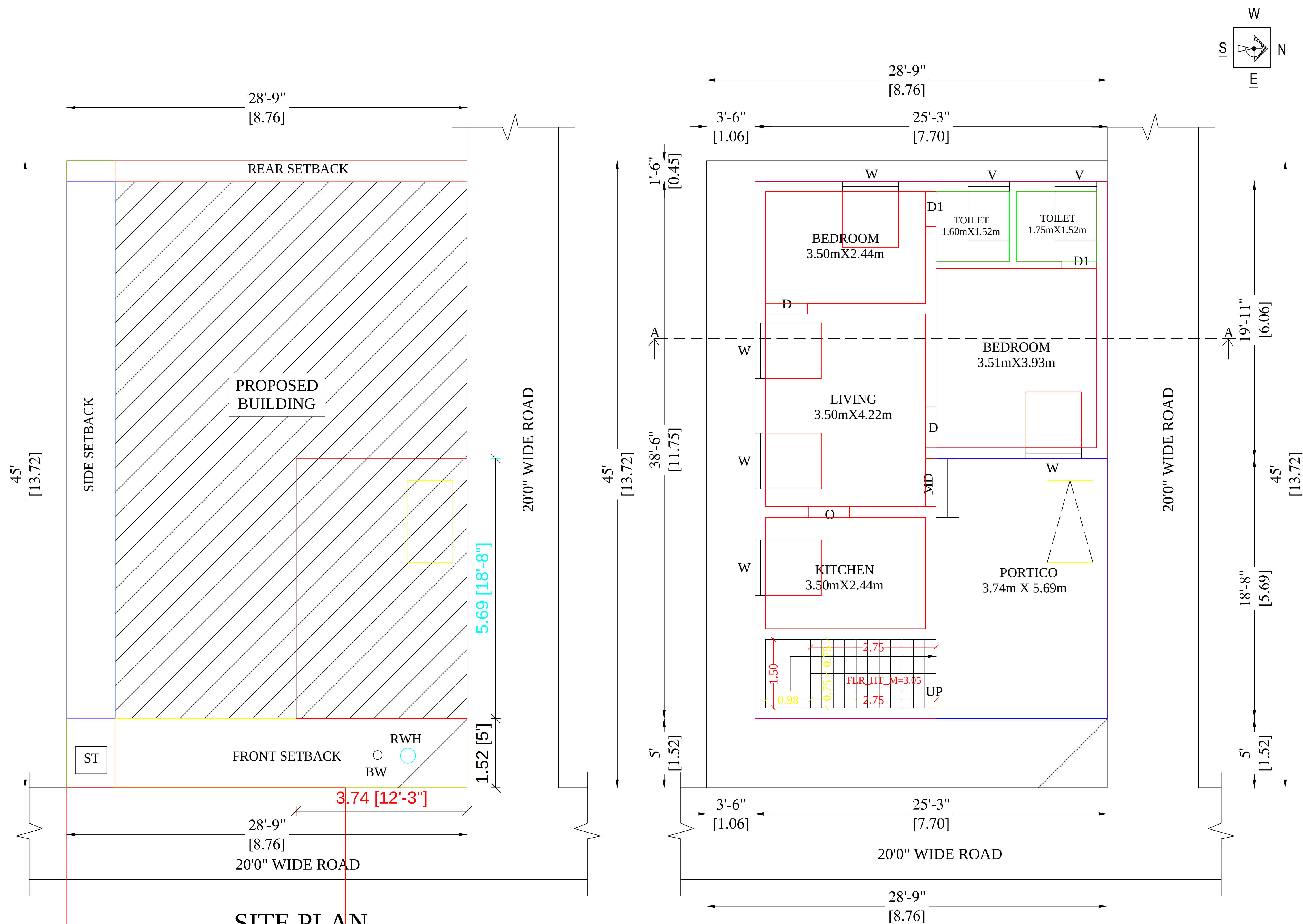
SITE PLAN
