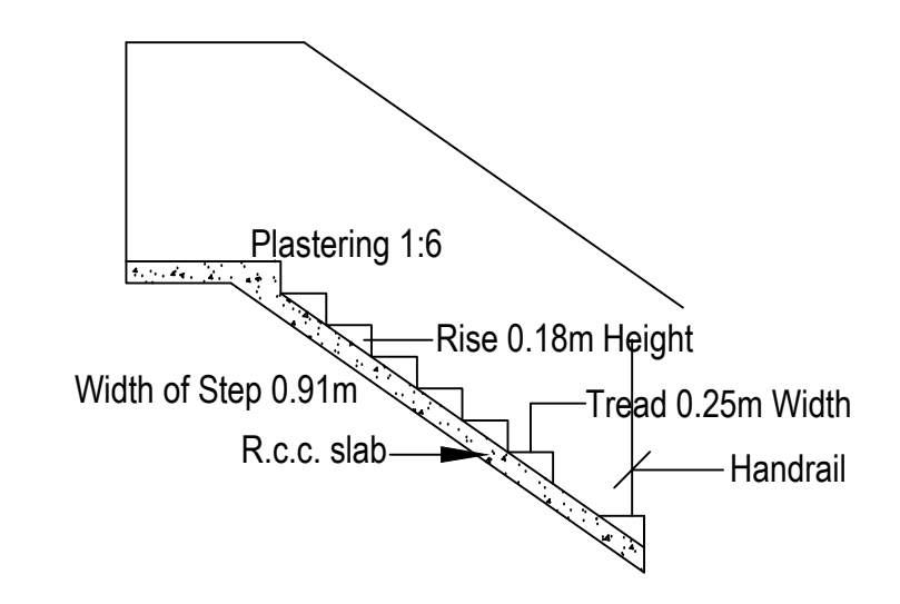
DETAILS OF STAIR CASE
