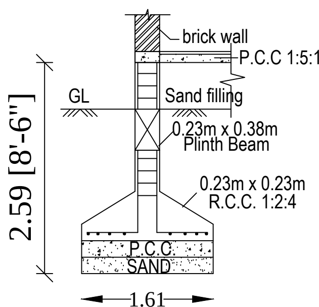
FOUNDATION DETAILS
