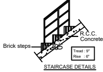
STAIRCASE DETAILS
