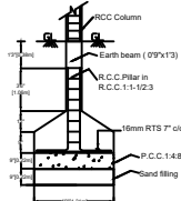
FOUNDATION DETAILS
