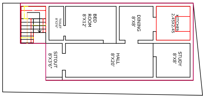
EXISTING GROUND FLOOR PLAN
