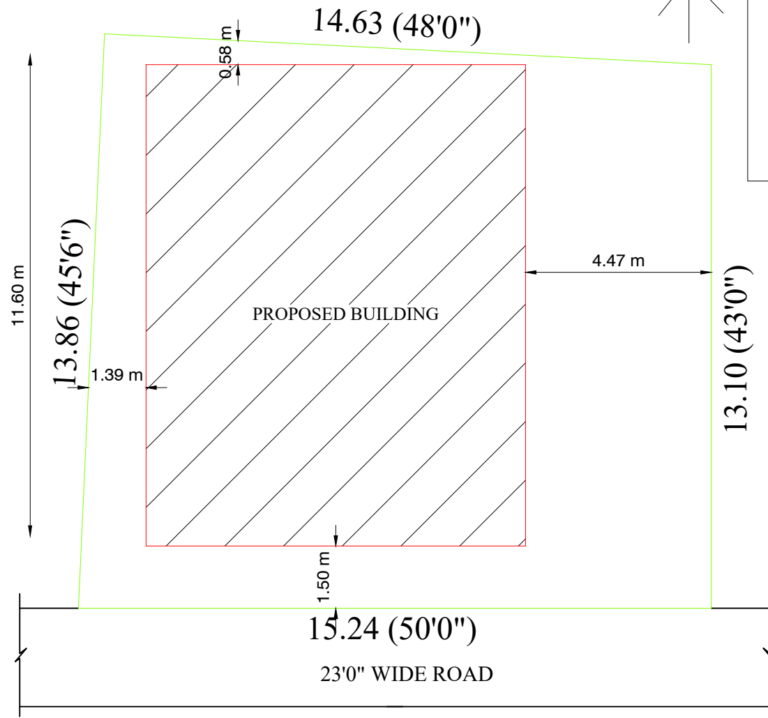
SITE PLAN
