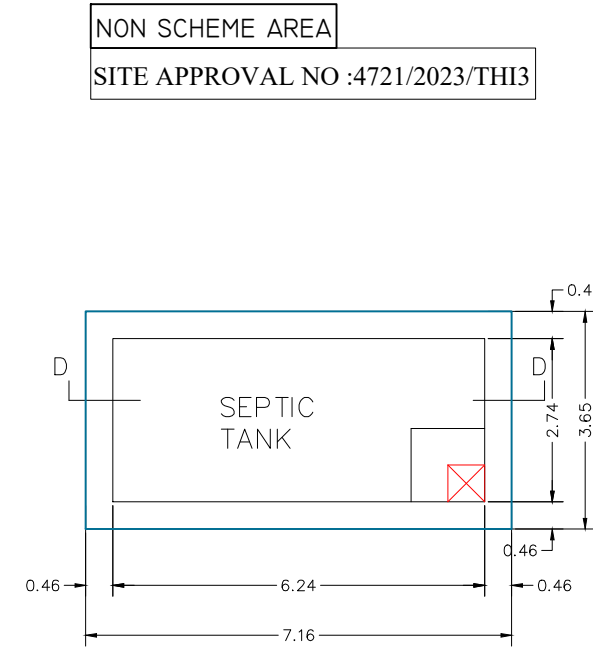
PLAN OF SEPTIC TANK SCALE 1"=2'-0"
