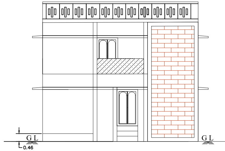
FRONT ELEVATION
