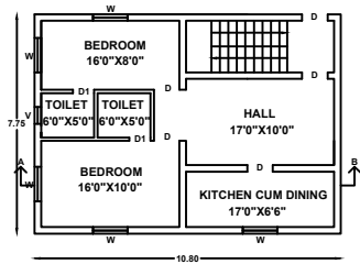
GROUND FLOOR PLAN
