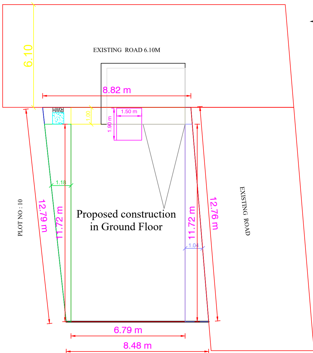
SITE PLAN
