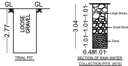
SECTION OF RAIN WATER COLLECTION PITS (NTS)
