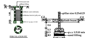
SEPTIC TANK DETAILS
