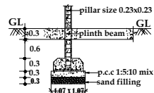
FOUNDATION DETAILS
