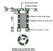
PERCOLATION PIT
