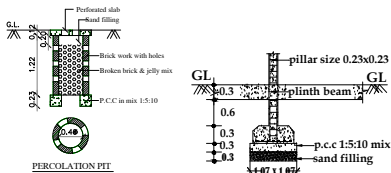
PERCOLATION PIT
