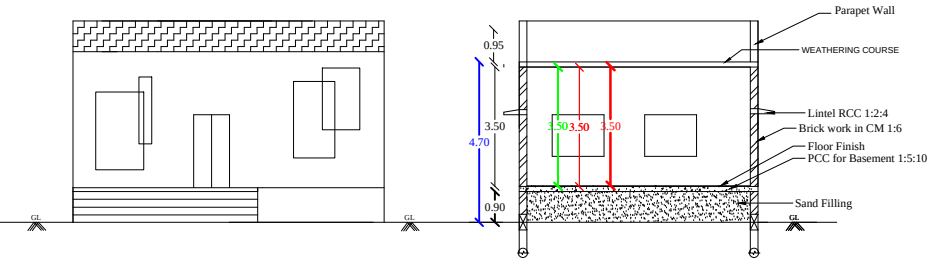
SECTION ON-AA
