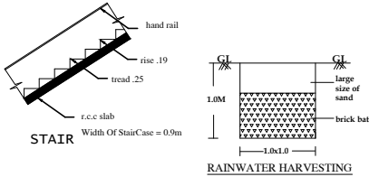
RAINWATER HARVESTING
