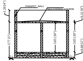
Section on-AA
