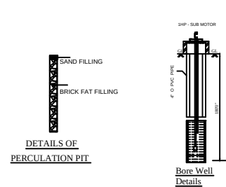
Bore Well Details
