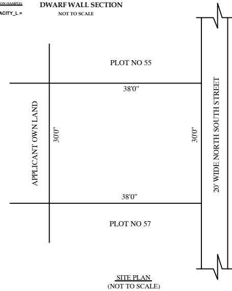
RWL_CAPACITY_L = 2000LTRS
