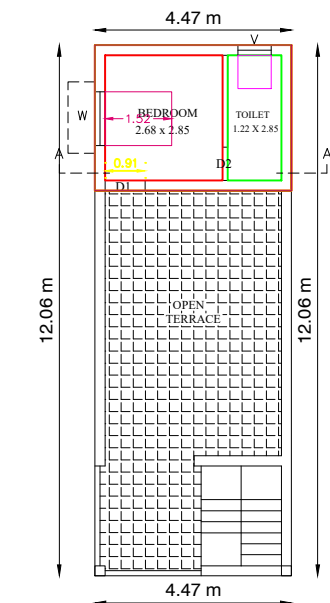
PRO.FIRST FLOOR PLAN
