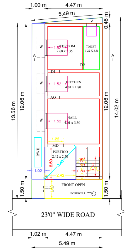
PRO.GROUND FLOOR PLAN
