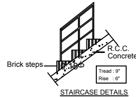
STAIRCASE DETAILS
