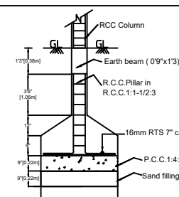
FOUNDATION DETAILS
