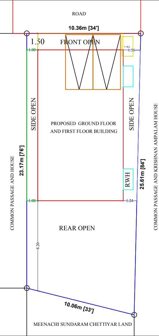
SITE PLAN
