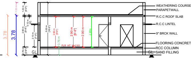
SECTION ON 'A-A'
