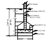
FOUNDATION DETAILS
