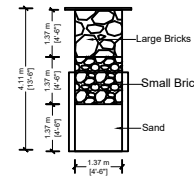
SECTION OF RAIN WATER COLLECTION PITS (NTS)
