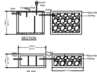
DETAILS OF SEPTIC TANK & DISPERSION TRENCH
