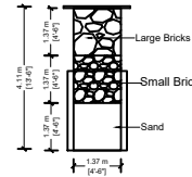
SECTION OF RAIN WATER COLLECTION PITS (NTS)
