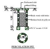
PERCOLATION PTT
