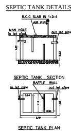
SEPTIC TANK DETAILS
