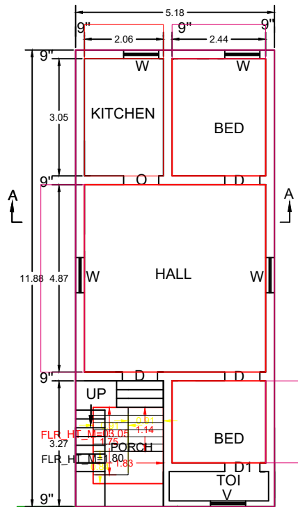
G.F. PLAN
