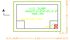
SUMP DETAIL
