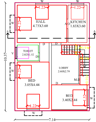
PRO.FIRST FLOOR PLAN
