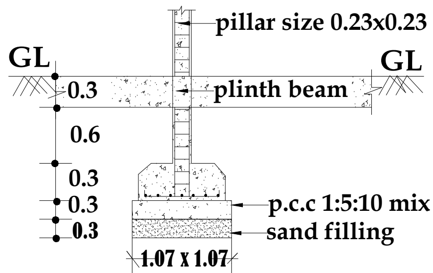
FOUNDATION DETAILS
