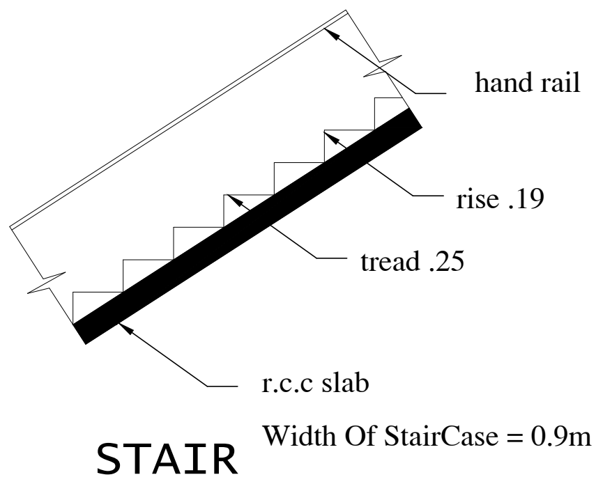
STAIR
