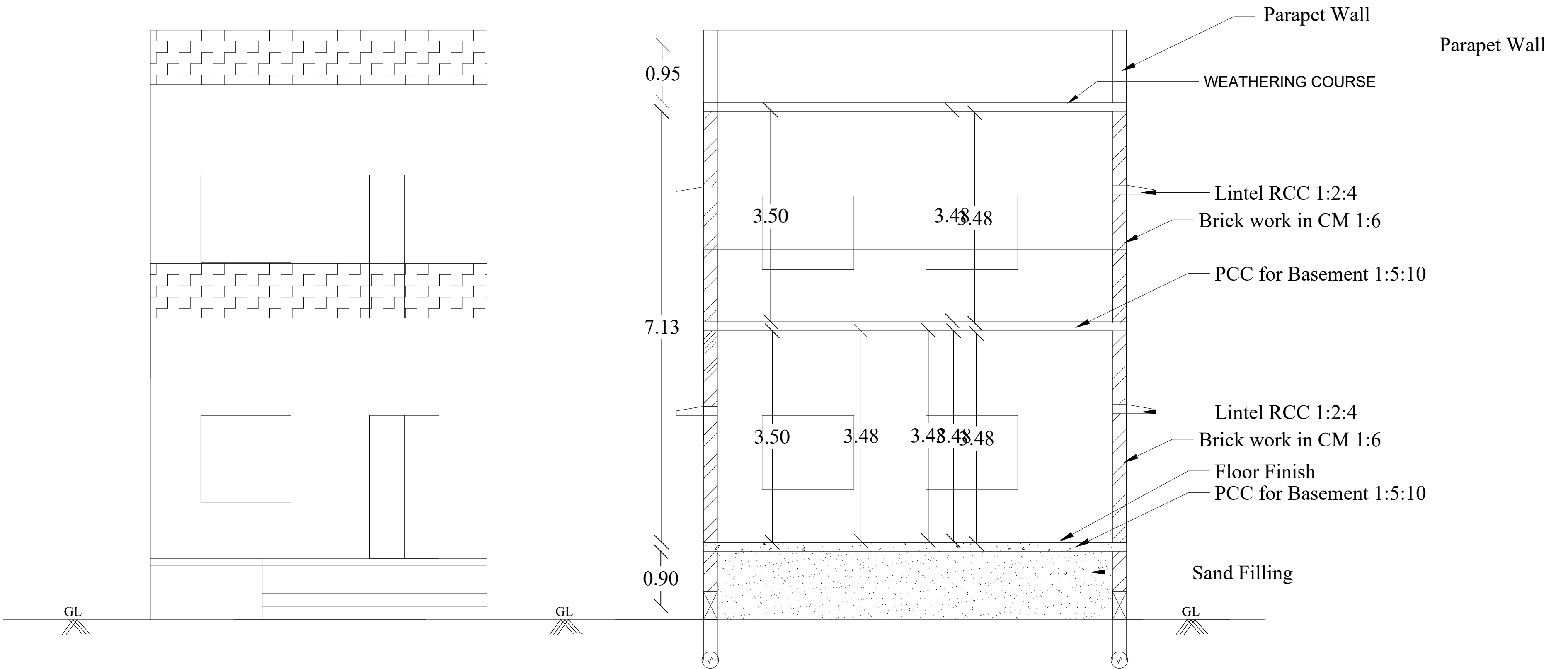
FRONT ELEVATION
