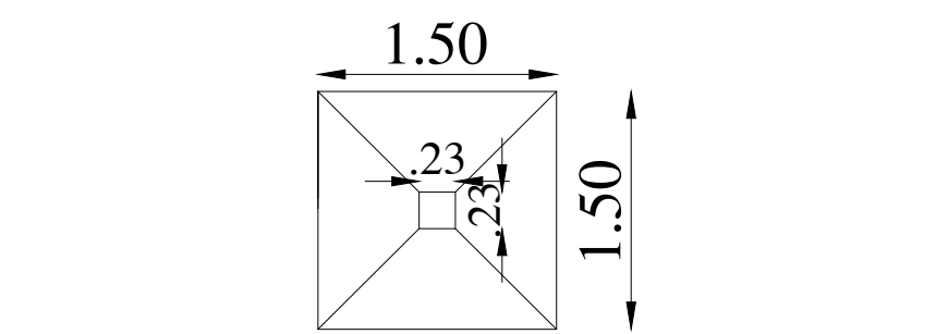
COLUMN FOUNDATION
