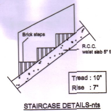
STAIRCASE DETAILS-nts
