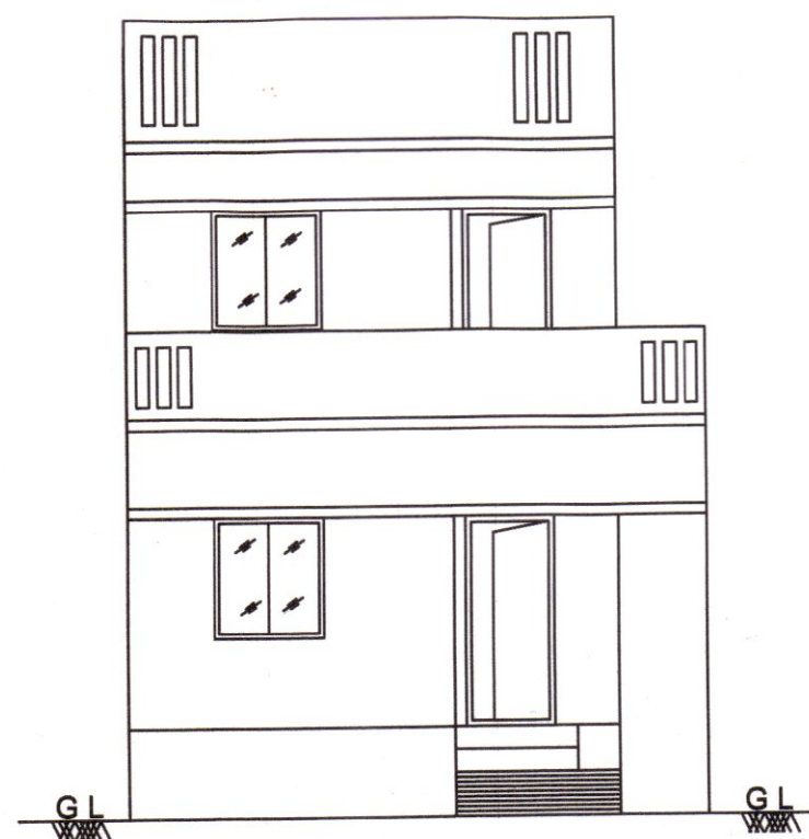
FRONT ELEVATION
