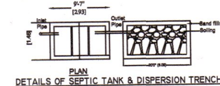
PLAN DETAILS OF SEPTIC TANK & DISPERSION TRENCH
