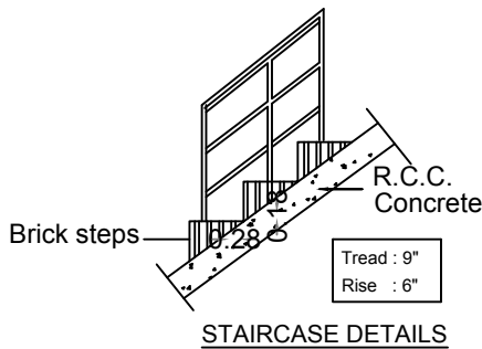
STAIRCASE DETAILS
