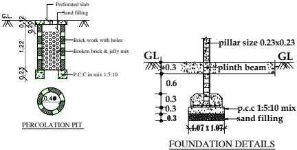
FOUNDATION DETAILS
