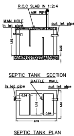
SEPTIC TANK DETAILS
