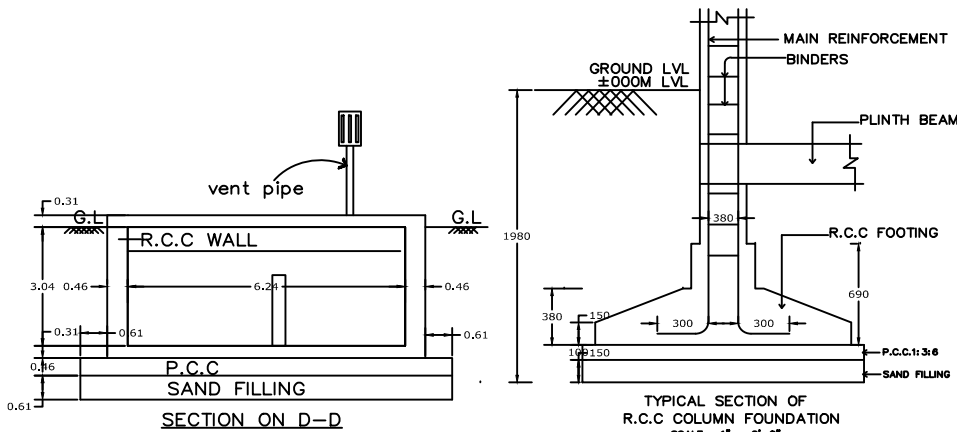
SECTION ON D-D
