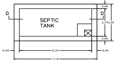
PLAN OF SEPTIC TANK SCALE 1"-2'0"
